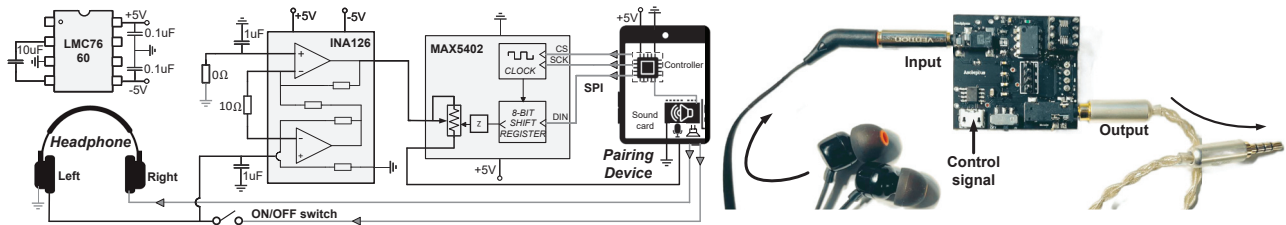
Figure 8: Schematic (left) and PCB (right) of Asclepius.
